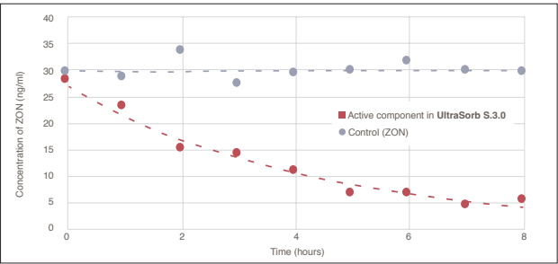
Figure 2. Biotransformation of ZON by UltraSorb S 3.0
